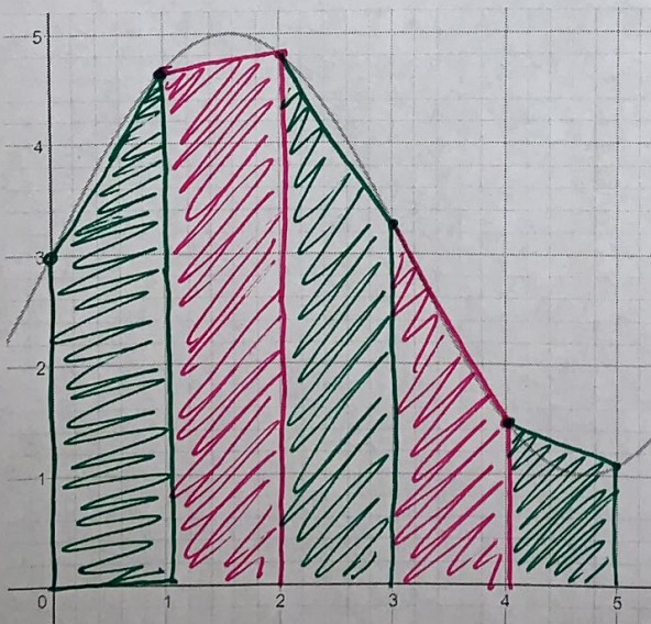
3. Trapezoid Method (5 subintervals)
