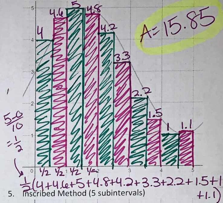
4. Right Riemann Sums (10 subintervals)
